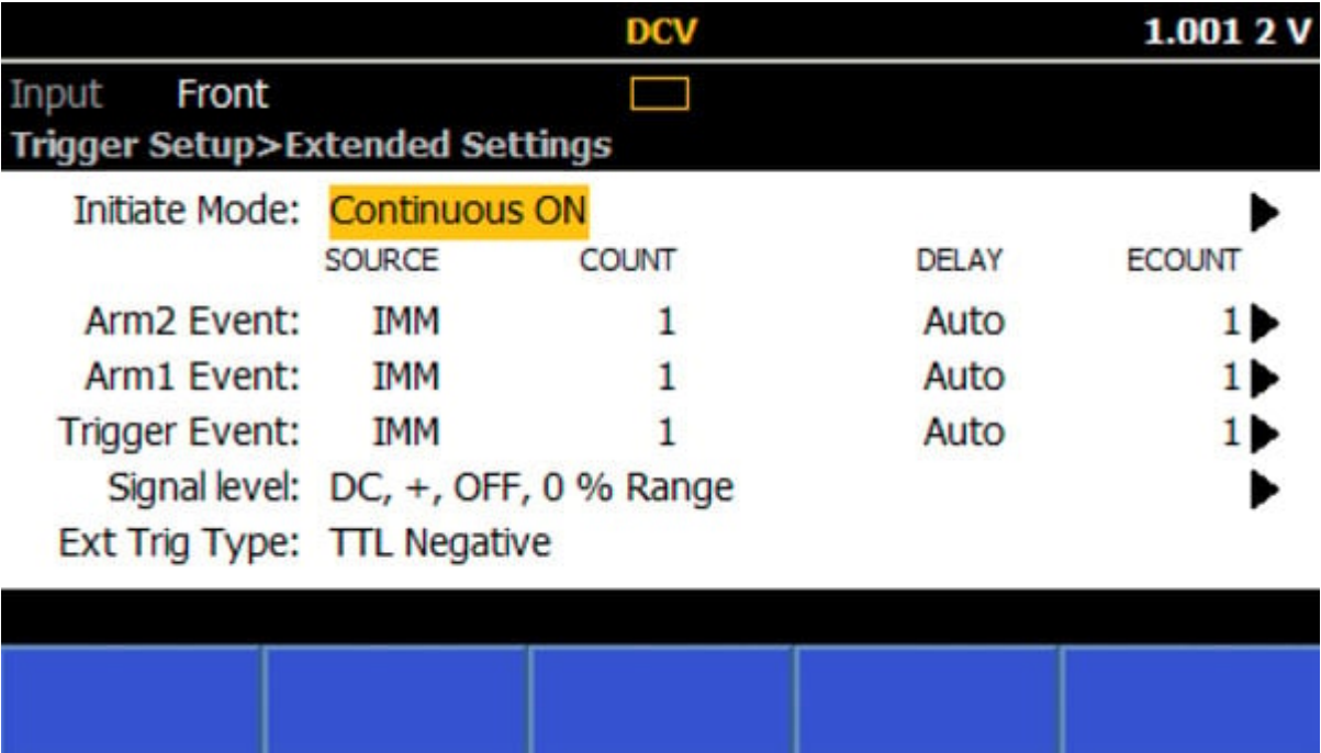
Trigger System
